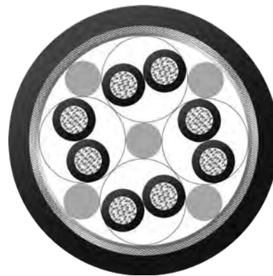
BizLink SeaLine® BWTS cable 4x2x0.75 VZN BK Order no.: L45551-D42-K16
